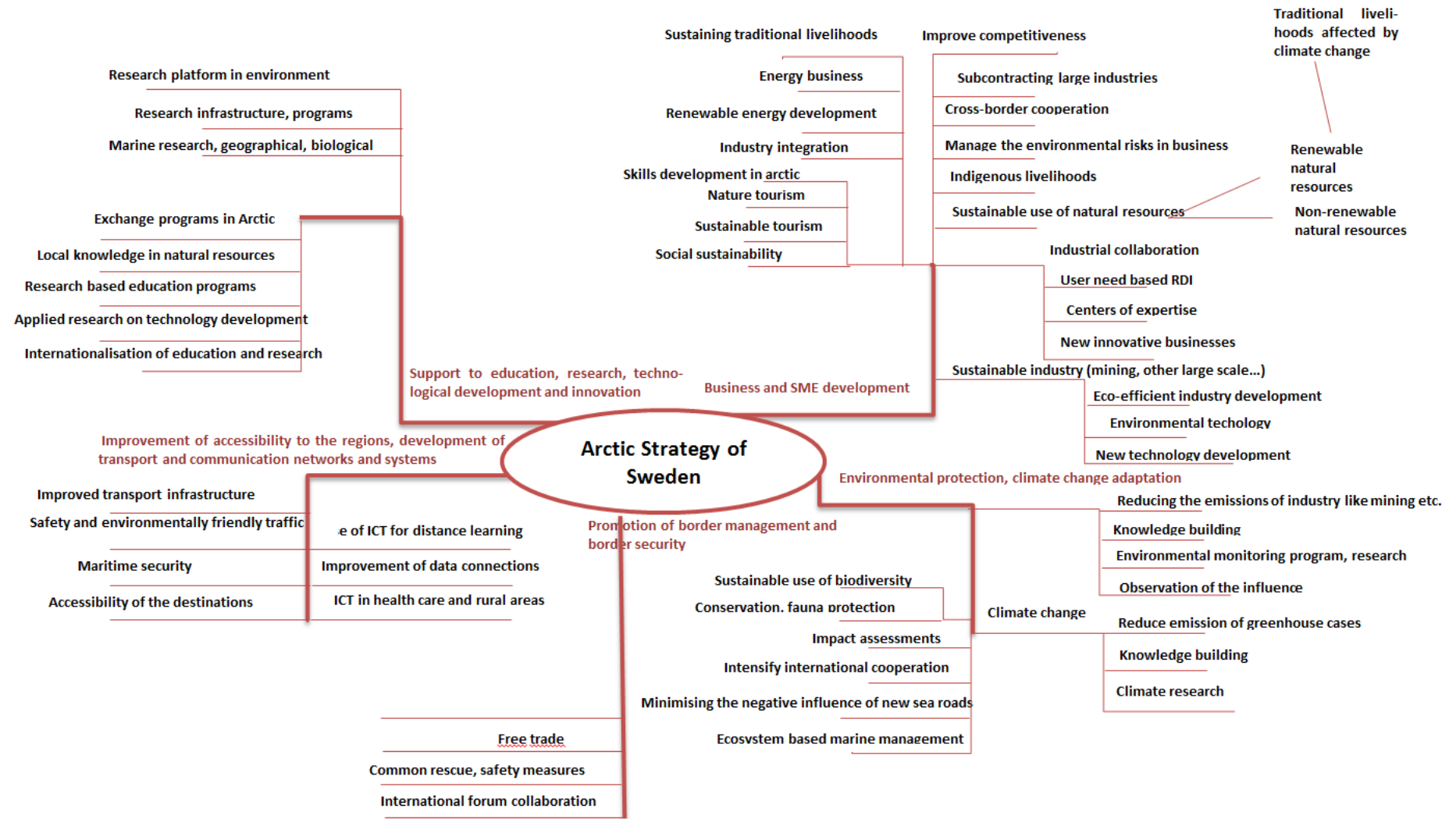
Figure 3. Mind Map
